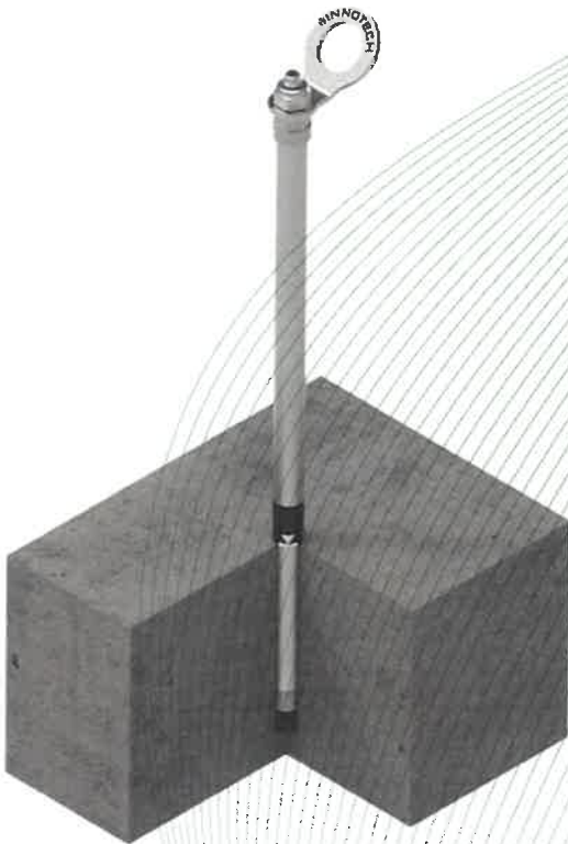
Fig. 1: Anchor device type A, type POINT-12
